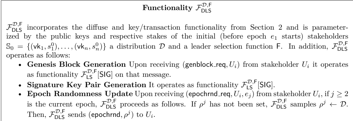
Figure 10: Functionality \mathcal{F}_{\text{DLS}}^{\mathcal{D},\text{F}} .
